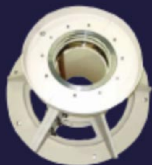
SXL TURBINE GUIDE BEARINGS WITH TAPARED KEYSET
