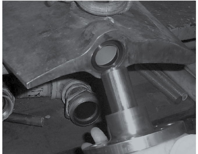
ThorPlas Wicket Gate Bearing with Thorseal
