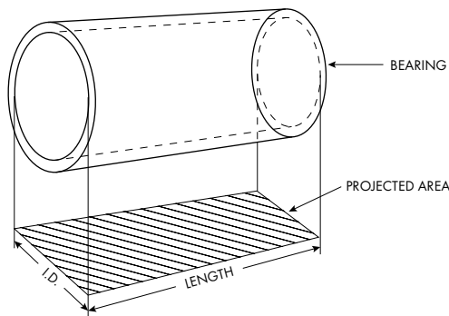
Figure 4: Bearing Pressure
