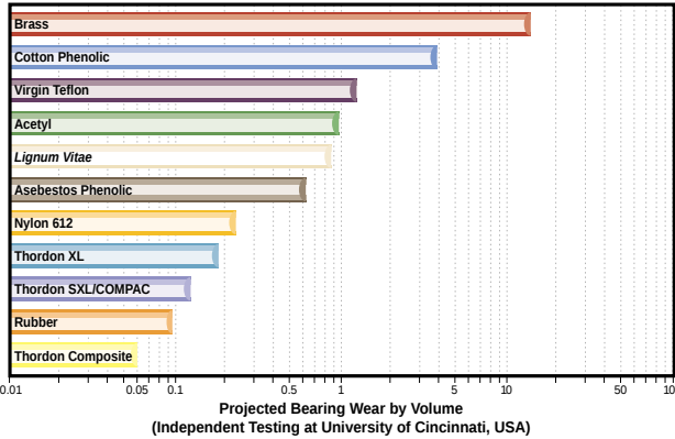
Typical Bearing Abrasive Wear Rates
